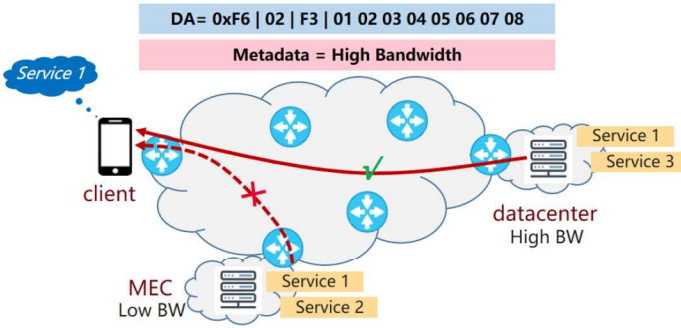
Fig. 3. Routing Based on Needs of Services.
